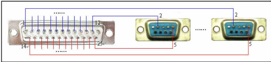
485 switch box and DVR connection
