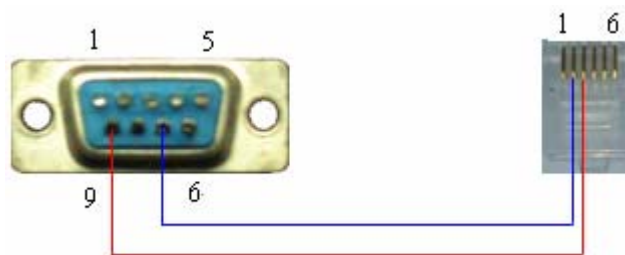
Keyboard and 485 switch box connection
