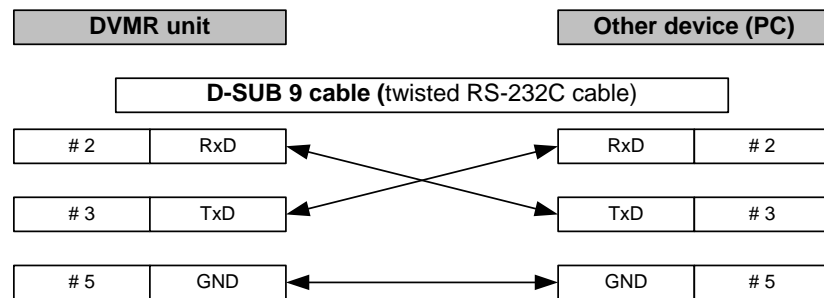
Connection to PC using RS-232C cable
